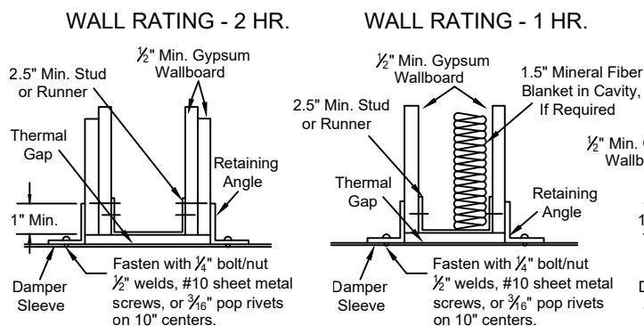
Fig. 1: Metal Stud/Gypsum Wall Design
