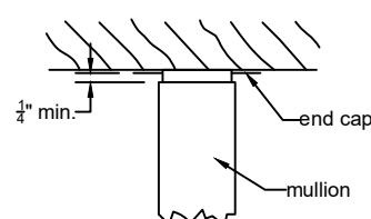
DETAIL G-G
