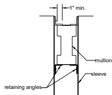
DETAIL E-E
