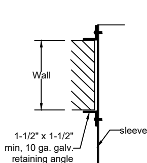
DETAIL D-D
