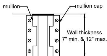
DETAIL F-F
