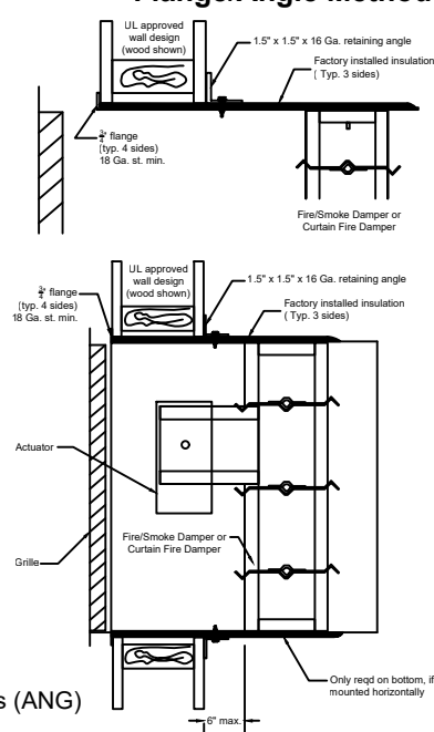
Fig. 2a - Grille Mount Flange/Angle Method
