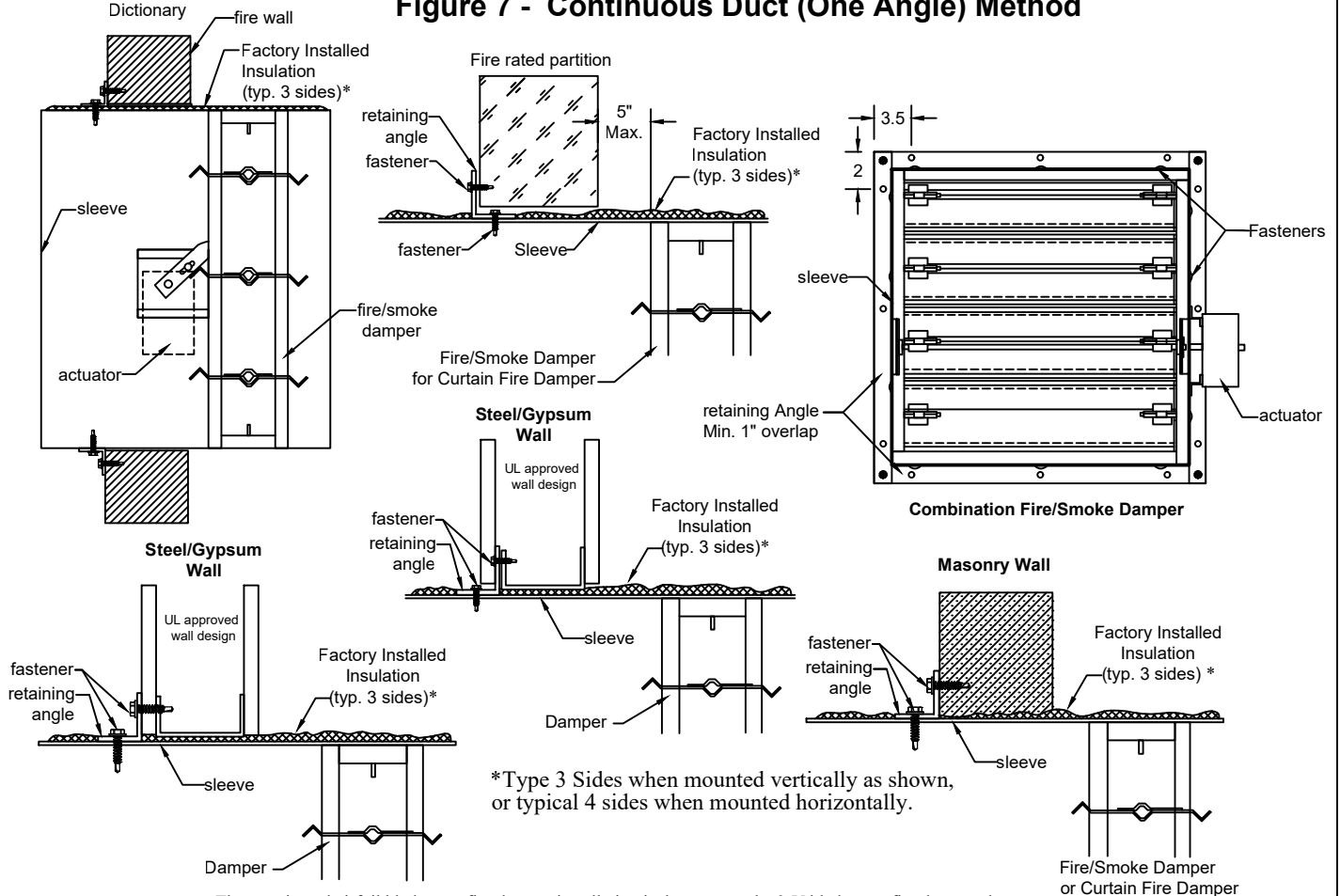
Figure 7 - Continuous Duct (One Angle) Method
