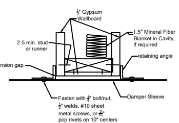
Fig. 1b: Wood Stud/Gypsum Design
