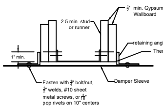
Fig. 1a: Metal Stud/Gypsum Design
