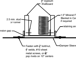
Fig. 1a: Metal Stud/Gypsum Design
