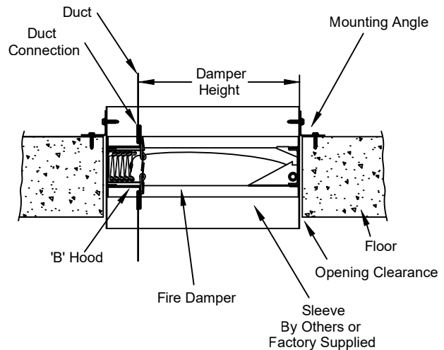
Horizontal Mount
