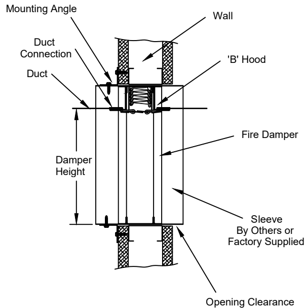
Vertical Mount
