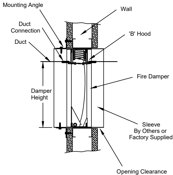
Vertical Mount
