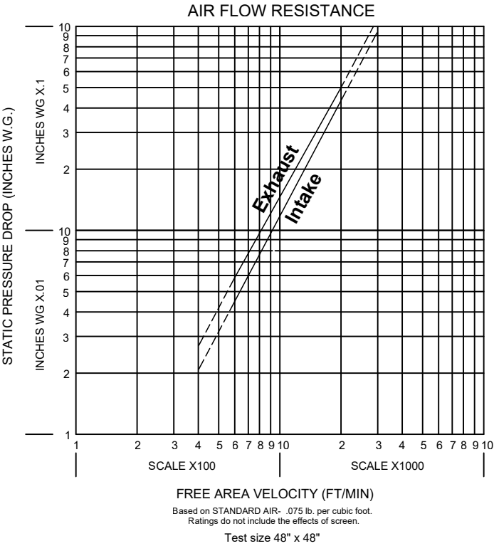
FL-D-6.1 FREE AREA IN SQ. FT.
