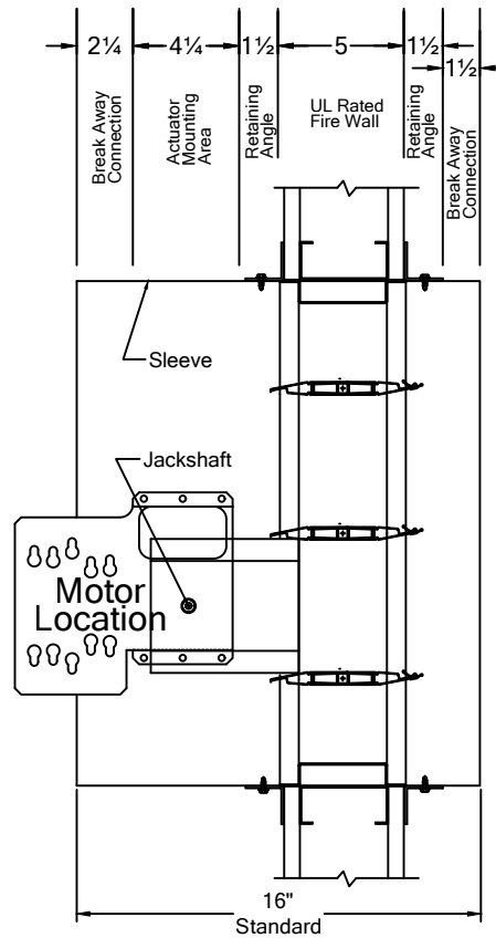
Damper Size 12 x 12
