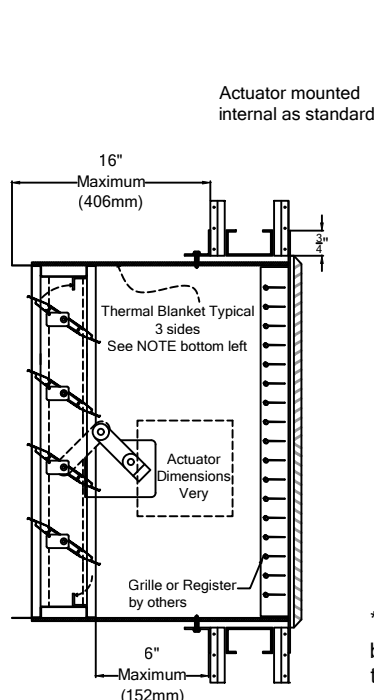
Metal Stud Installation
