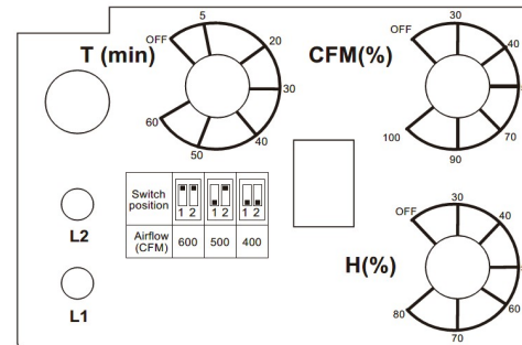
Built-in control panel
