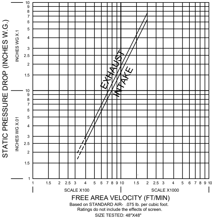
AMCA Figure 5.5
